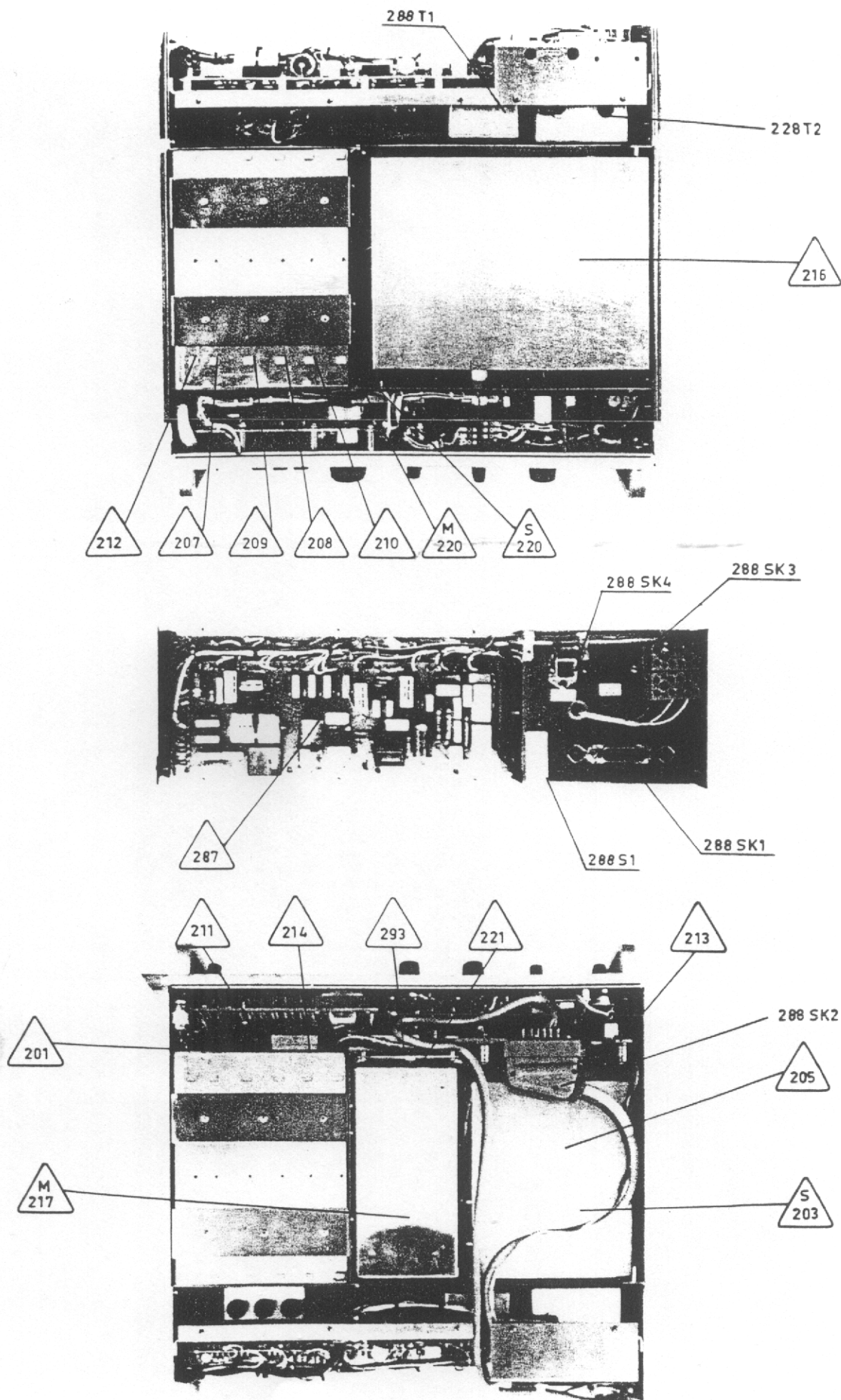
LOCATION OF CIRCUIT BOARDS RECEIVER 5000 S1
